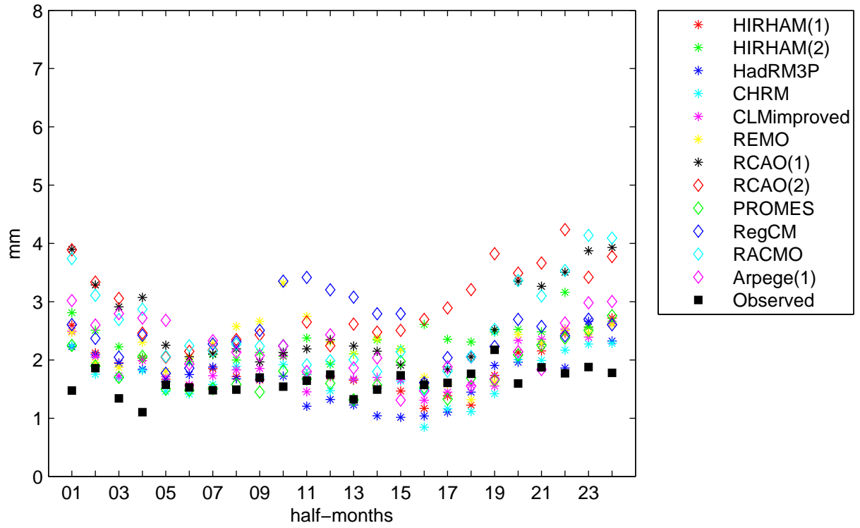
Heathrow Control 1961–1990 Mean Precipitation
