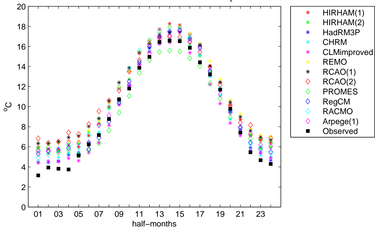
Gatwick Control 1961–1990 Mean Air Temperature
