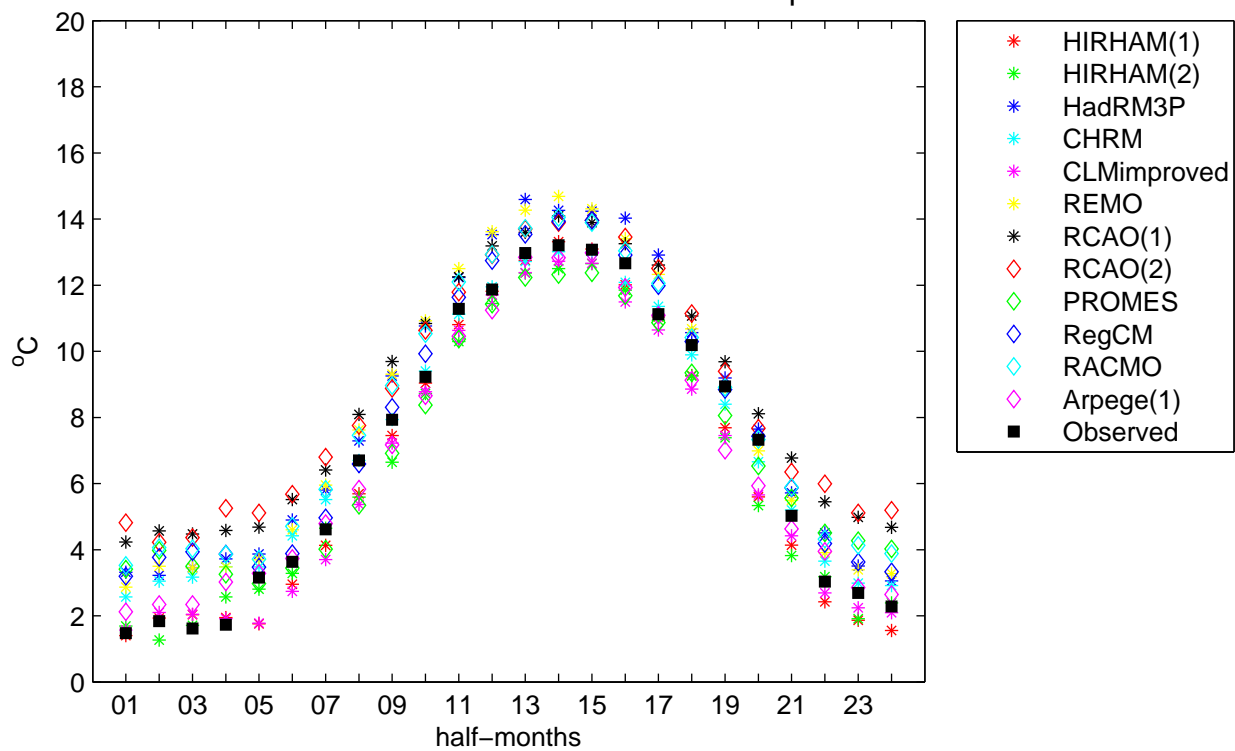
Eskdalemuir Control 1961–1990 Mean Air Temperature
