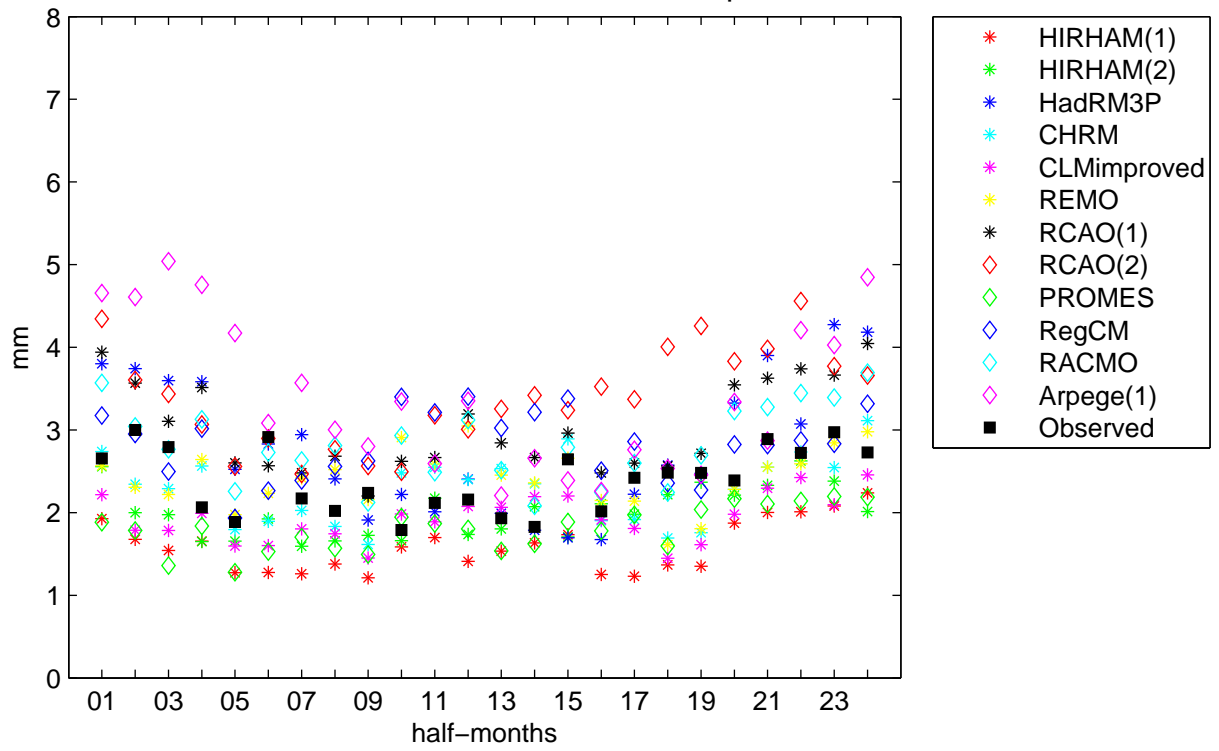
Bradford Control 1961–1990 Mean Precipitation
