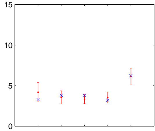
Heatwave duration
