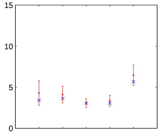
Heatwave duration
