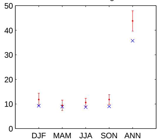
Number of "Cold nights"
