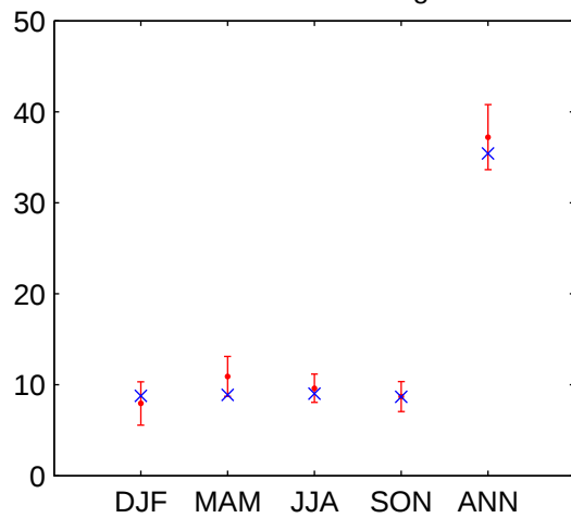
Number of "Warm nights"
