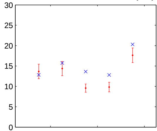
Maximum number of consecutive dry days
