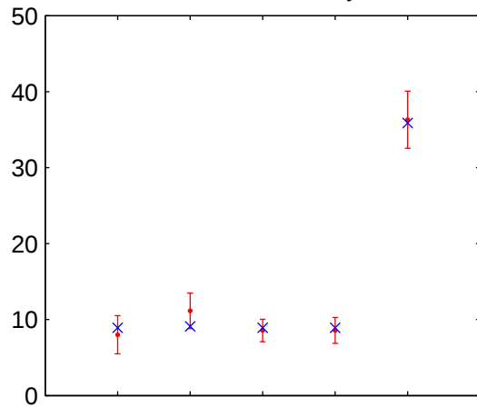
Number of "Hot days"
