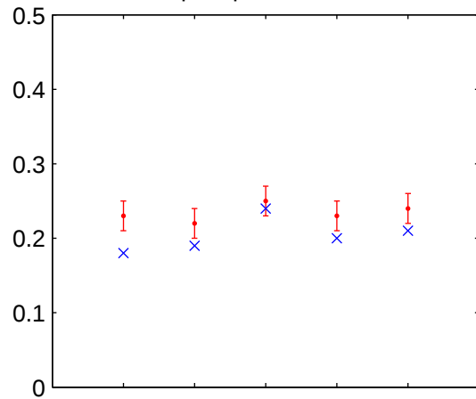
Fraction of total precipitation from intense events
