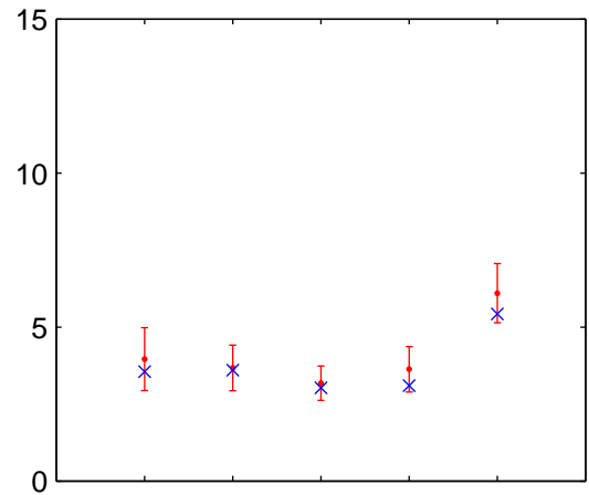
Heatwave duration
