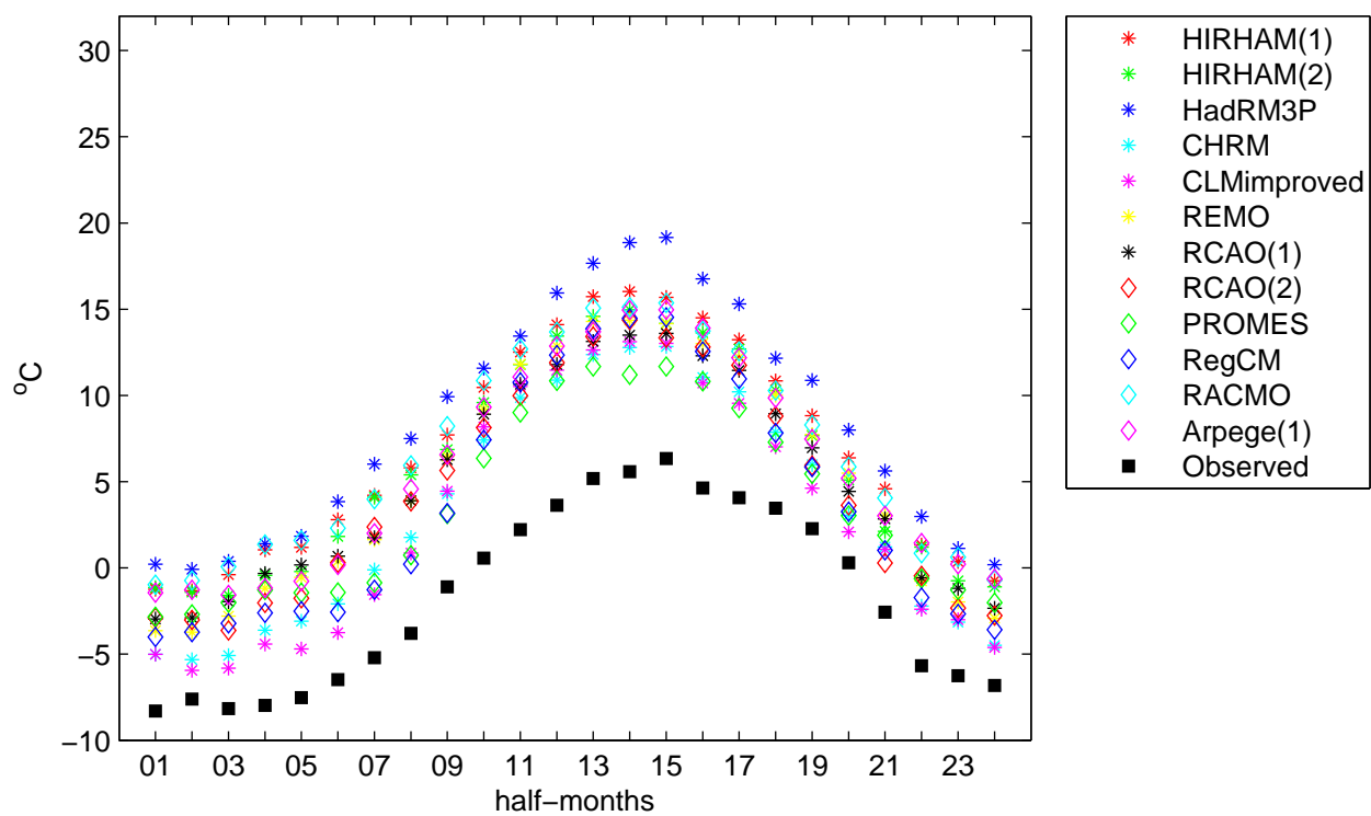
Saentis Control 1961–1990 Mean Air Temperature
