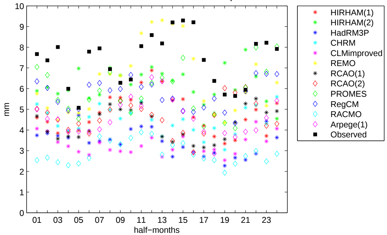
Saentis Control 1961–1990 Mean Precipitation
