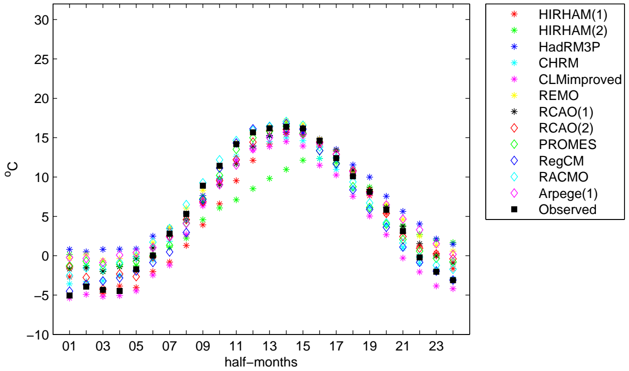
Karlstad Control 1961–1990 Mean Air Temperature
