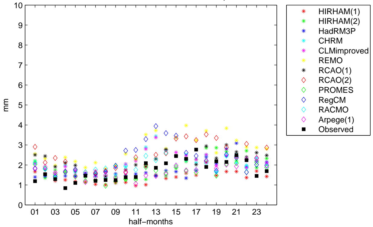
Karlstad Control 1961–1990 Mean Precipitation
