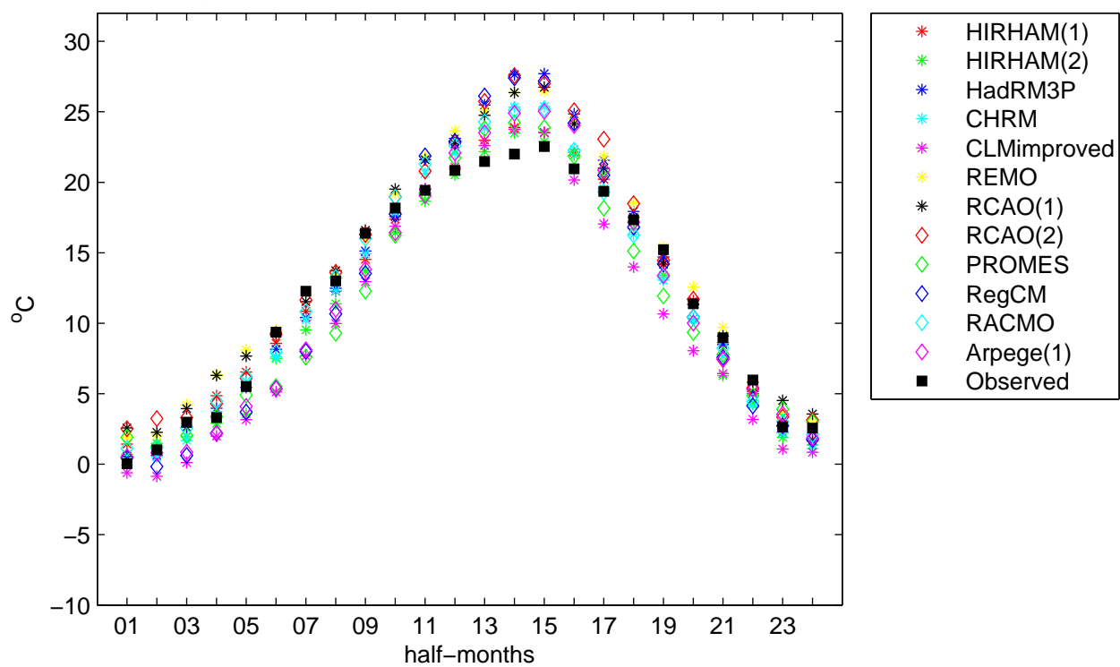
Beograd Control 1961–1990 Mean Air Temperature
