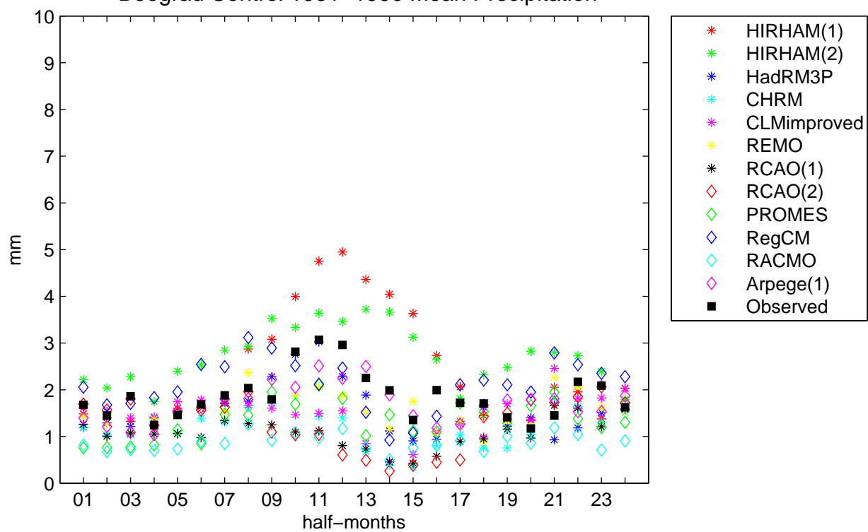
Beograd Control 1961–1990 Mean Precipitation
