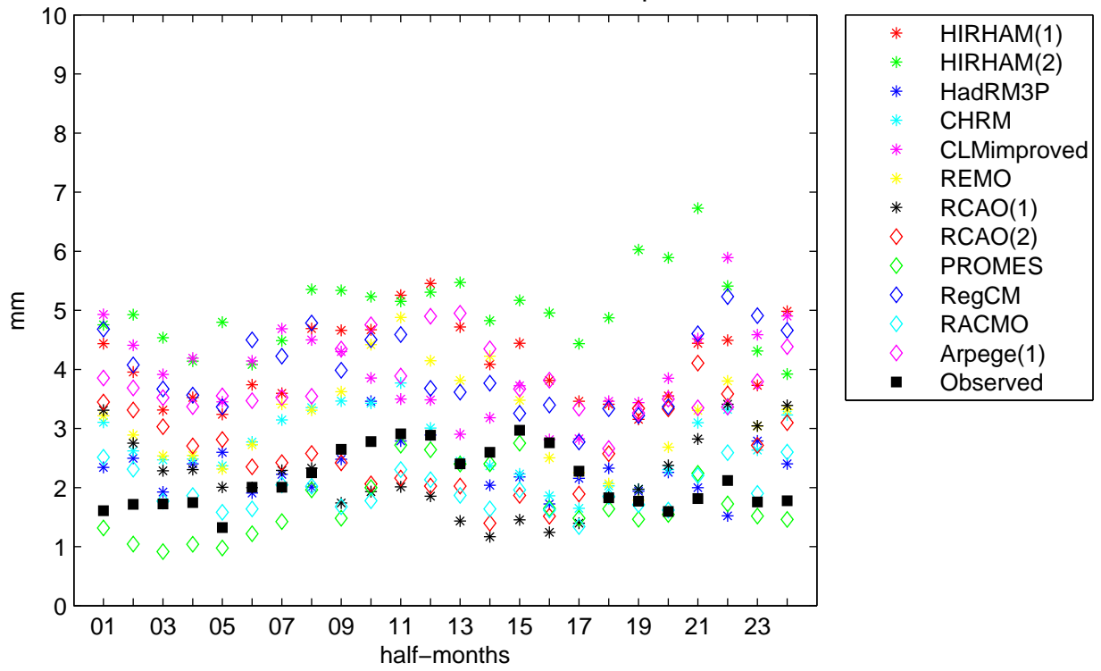
Basel Control 1961–1990 Mean Precipitation
