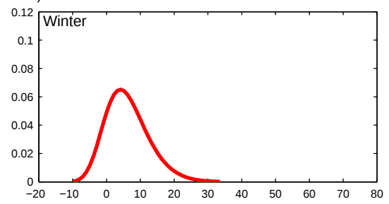
Beograd A2 scenario Probability density of getting a certain change in heatwave duration Heavy red line: scenario period (2071–2100) – ensemble mean Coloured lines: scenario period (2071–2100) – ensemble members
