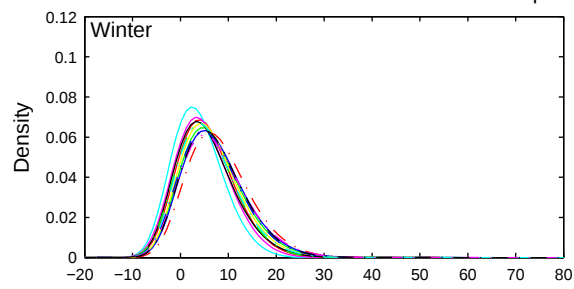
Beograd A2 scenario Probability density of getting a certain change in heatwave duration Heavy red line: scenario period (2071–2100) – ensemble mean Coloured lines: scenario period (2071–2100) – ensemble members
