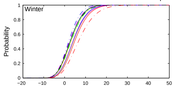
Karlstad A2 scenario Cumulative probability of getting a certain change in heatwave duration Heavy red line: scenario period (2071–2100) – ensemble mean Coloured lines: scenario period (2071–2100) – ensemble members
