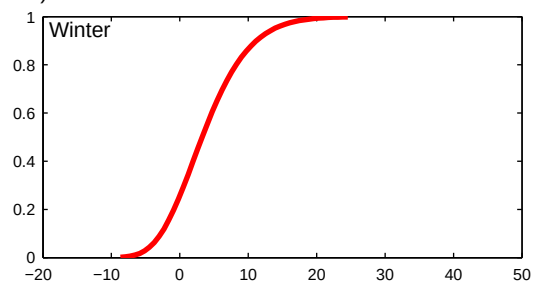
Karlstad A2 scenario Cumulative probability of getting a certain change in heatwave duration Heavy red line: scenario period (2071–2100) – ensemble mean Coloured lines: scenario period (2071–2100) – ensemble members
