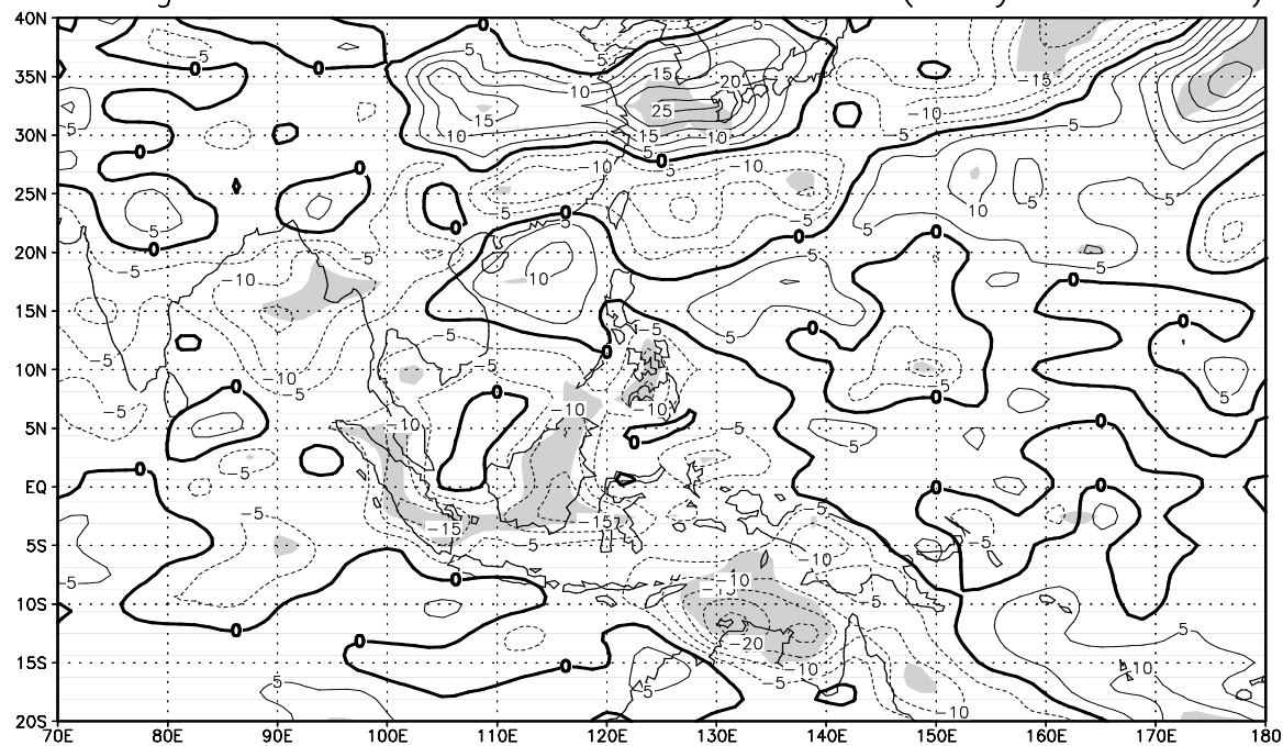
Figure 9.16: Change in net down surface radiation (Wm -2 ) in January (a) and July (b). Areas in which changes are locally significant at the 5% level are shaded.
