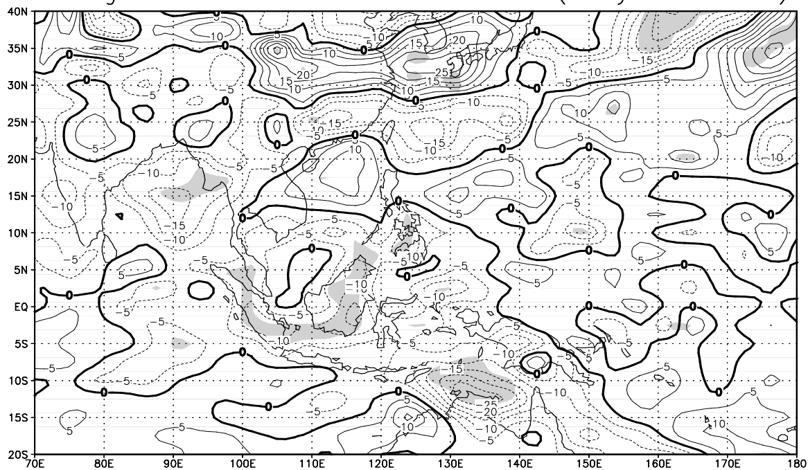
Figure 9.14: Change in net down surface short-wave radiation ( \text{Wm}^{-2} ) in January (a) and July (b). Areas in which changes are locally significant at the 5% level are shaded.
