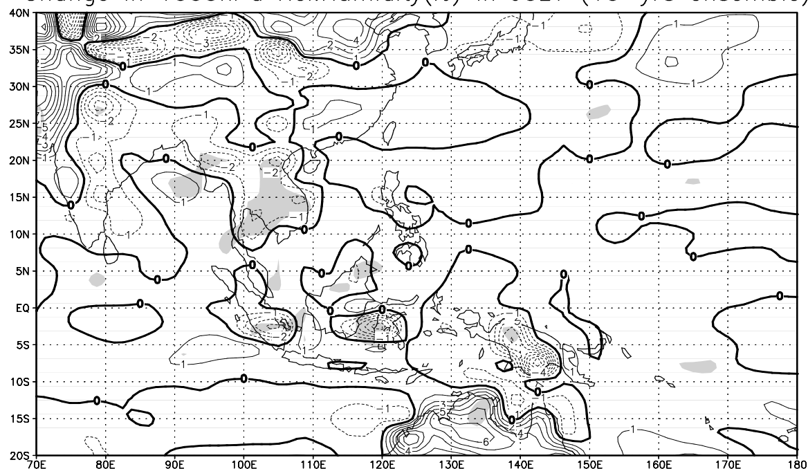
Figure 9.13: Change in 1000 hPa relative humidity (%) in January (a) and July (b). Areas in which changes are locally significant at the 5% level are shaded.
