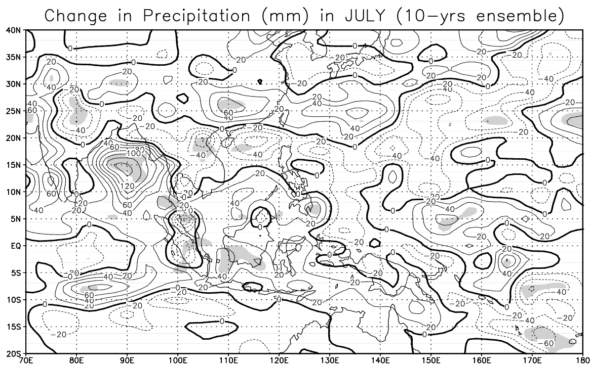
Figure 9.11: Change in total precipitation (mm) in January (a) and July (b). Areas in which changes are locally significant at the 5% level are shaded.
