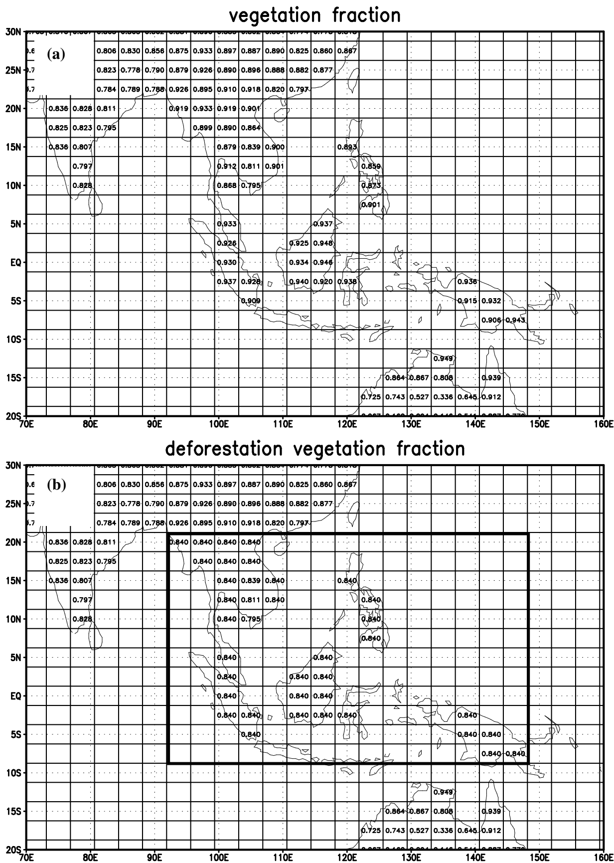
Figure 8.8: As in Figure 8.3 but for vegetation fraction.
