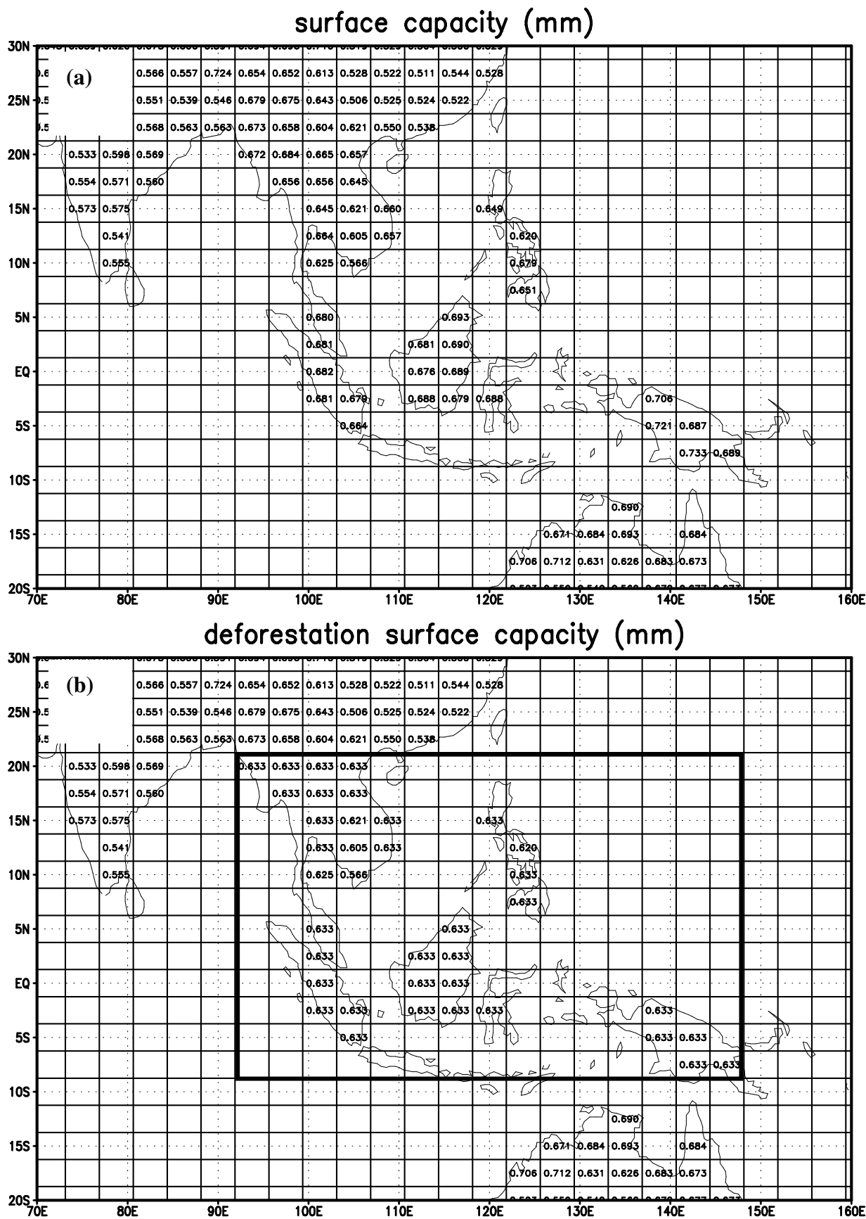
Figure 8.7: As in Figure 8.3 but for surface capacity (mm).
