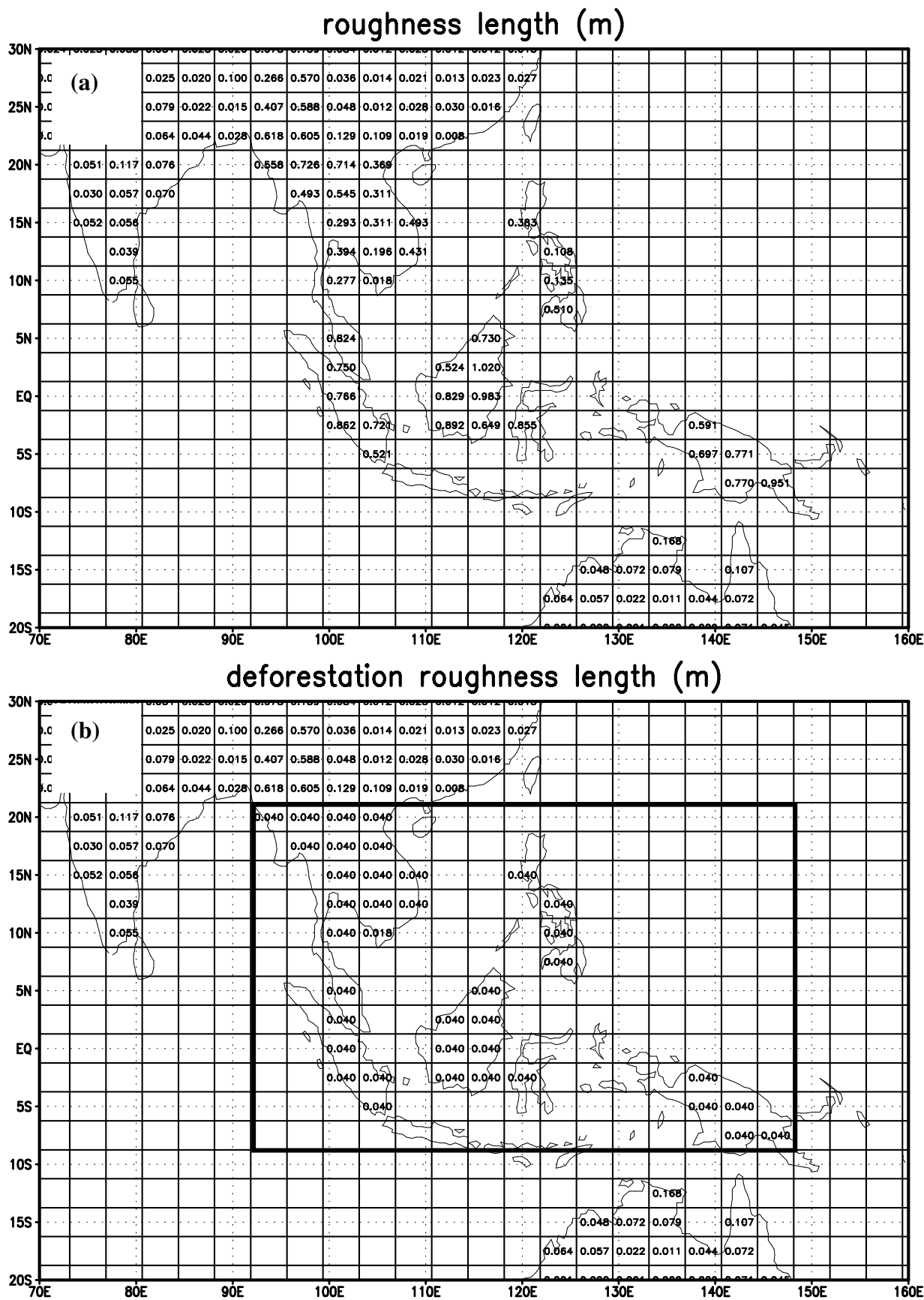
Figure 8.6: As in Figure 8.3 but for roughness length (m).
