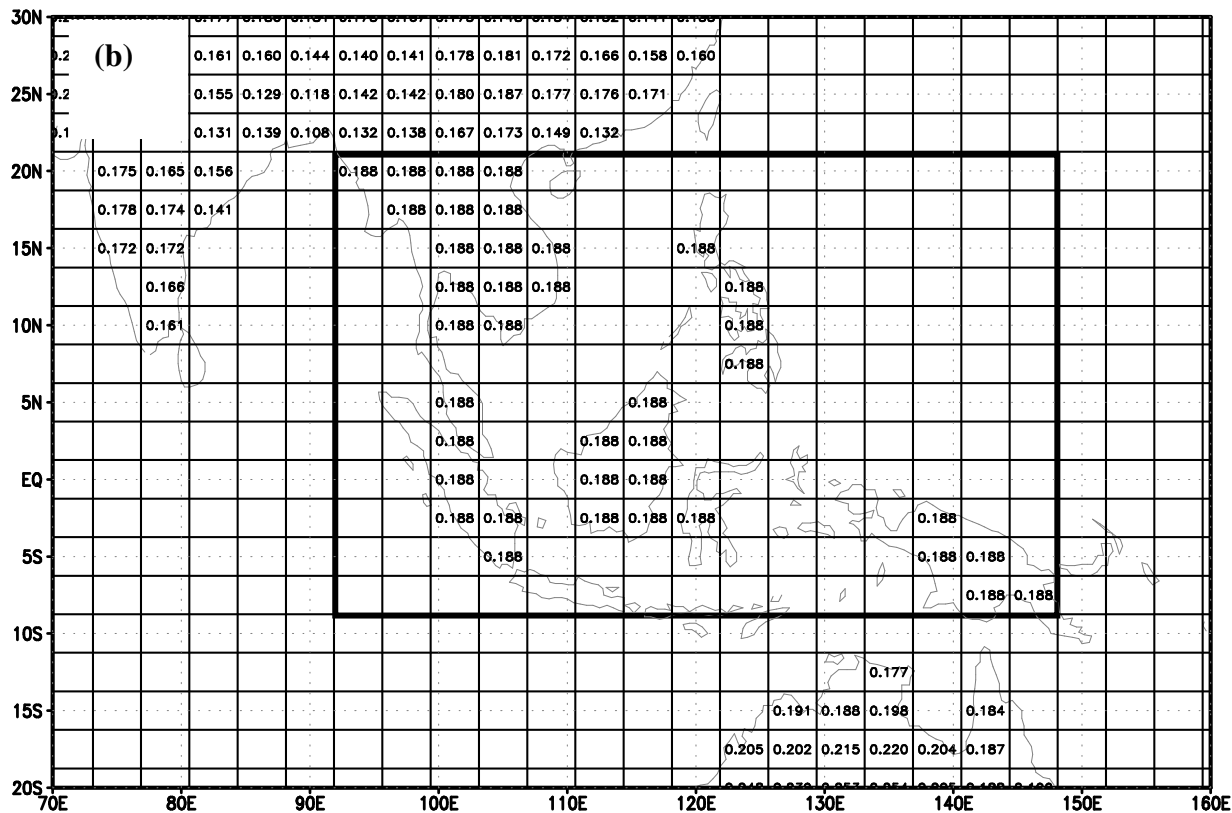
Figure 8.4: As in Figure 8.3 but for snow-free albedo.
