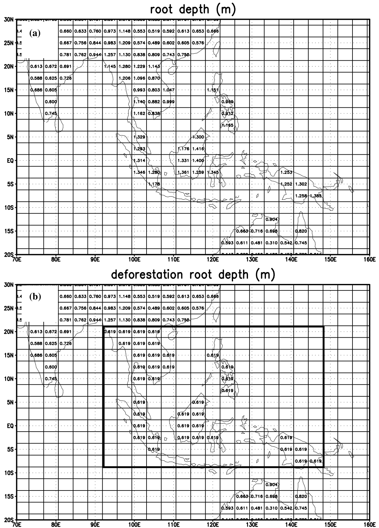
Figure 8.3: Root depth for the control (a) and deforestation (b) experiments. The inner box in (b) is the study area enclosing the deforested region (i.e. grid-boxes with a new value).
