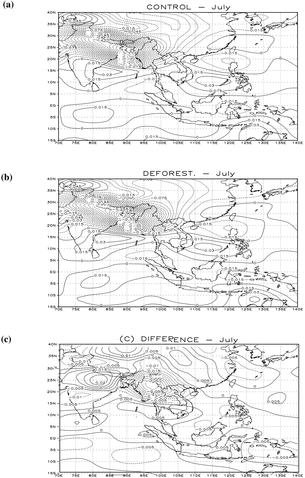
Figure 5.14: Change of vertical velocity near surface ( \text{Pa s}^{-1} ) in July.
