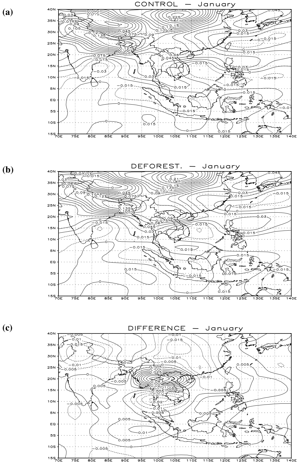
Figure 5.13: Change of vertical velocity near surface ( \text{Pa s}^{-1} ) in January.
