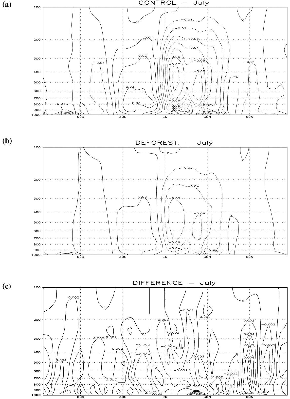
Figure 5.12: Change of Hadley circulation (zonal average of vertical velocity from 90°E to 130°E) ( \text{Pa s}^{-1} ) in July.
