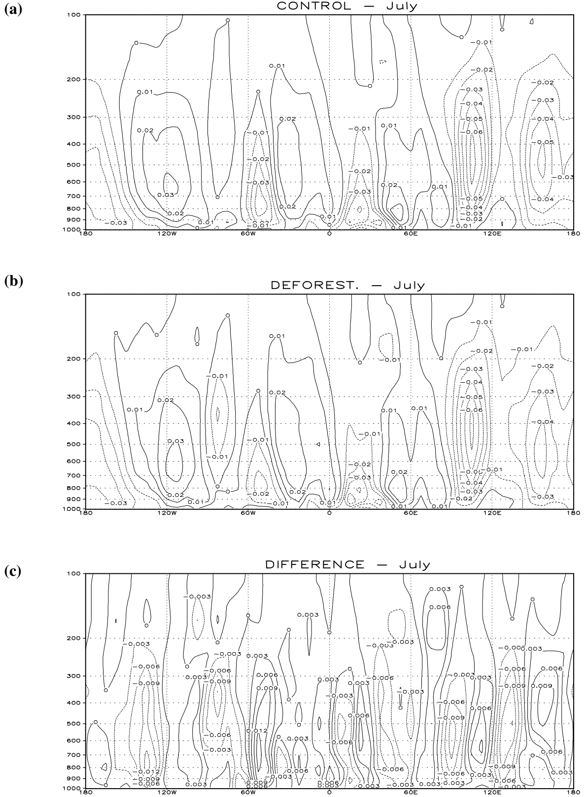
Figure 5.10: Change of Walker circulation (meridional average of vertical velocity from 15°S to 15°N) ( \text{Pa s}^{-1} ) in July.
