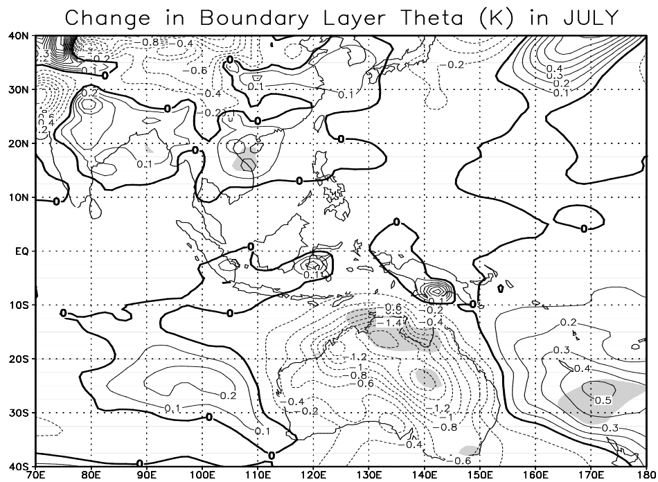
Figure 10.21: Change in boundary layer potential temperature, \Pi , (K) in January (a) and July (b). Changes locally significant at the 5% level are shaded (composite from 10-case ensemble).
