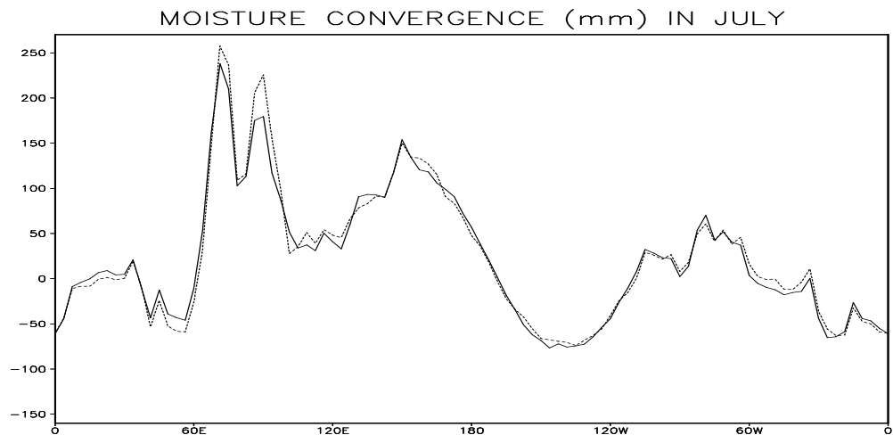
Figure 10.17: The zonal distribution of surface moisture flux, precipitation and moisture convergence (mm) in July for the control (solid line) and deforestation (dotted line) (meridionally averaged from 10°S to 20°N, 10-case ensemble).
