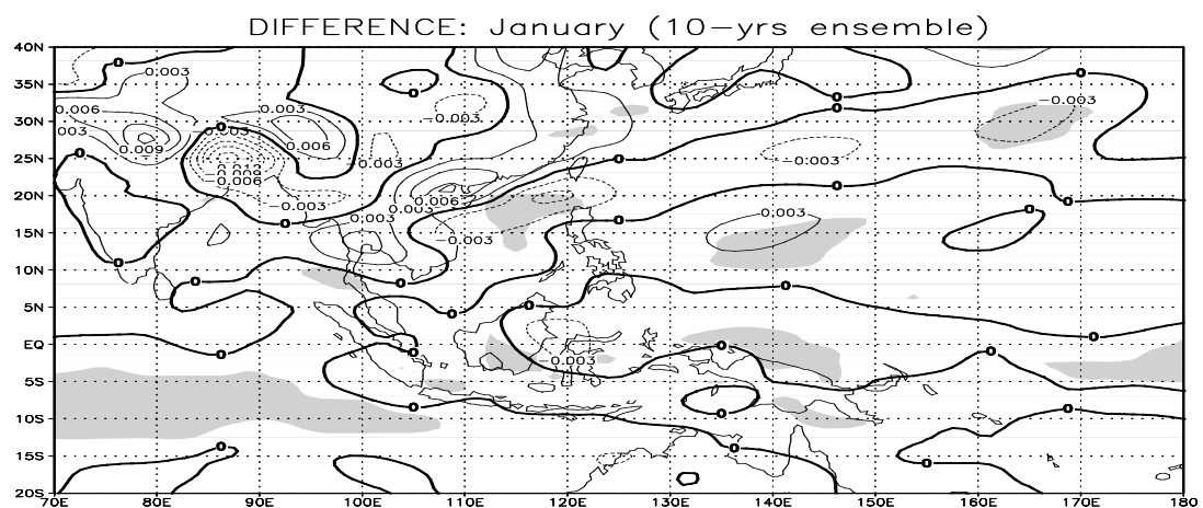
Figure 10.6: Change in vertical velocity pattern at lower level (850 hPa) (Pa/s) in January. Changes locally significant at the 5% level are shaded.
