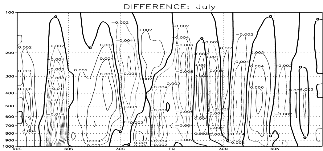
Figure 10.4: Change of Hadley circulation (zonal average of vertical velocity from 90^{\circ}\text{E} to 150^{\circ}\text{E} ) ( \text{Pa/s} ) in July (composite from 10-case ensemble).
