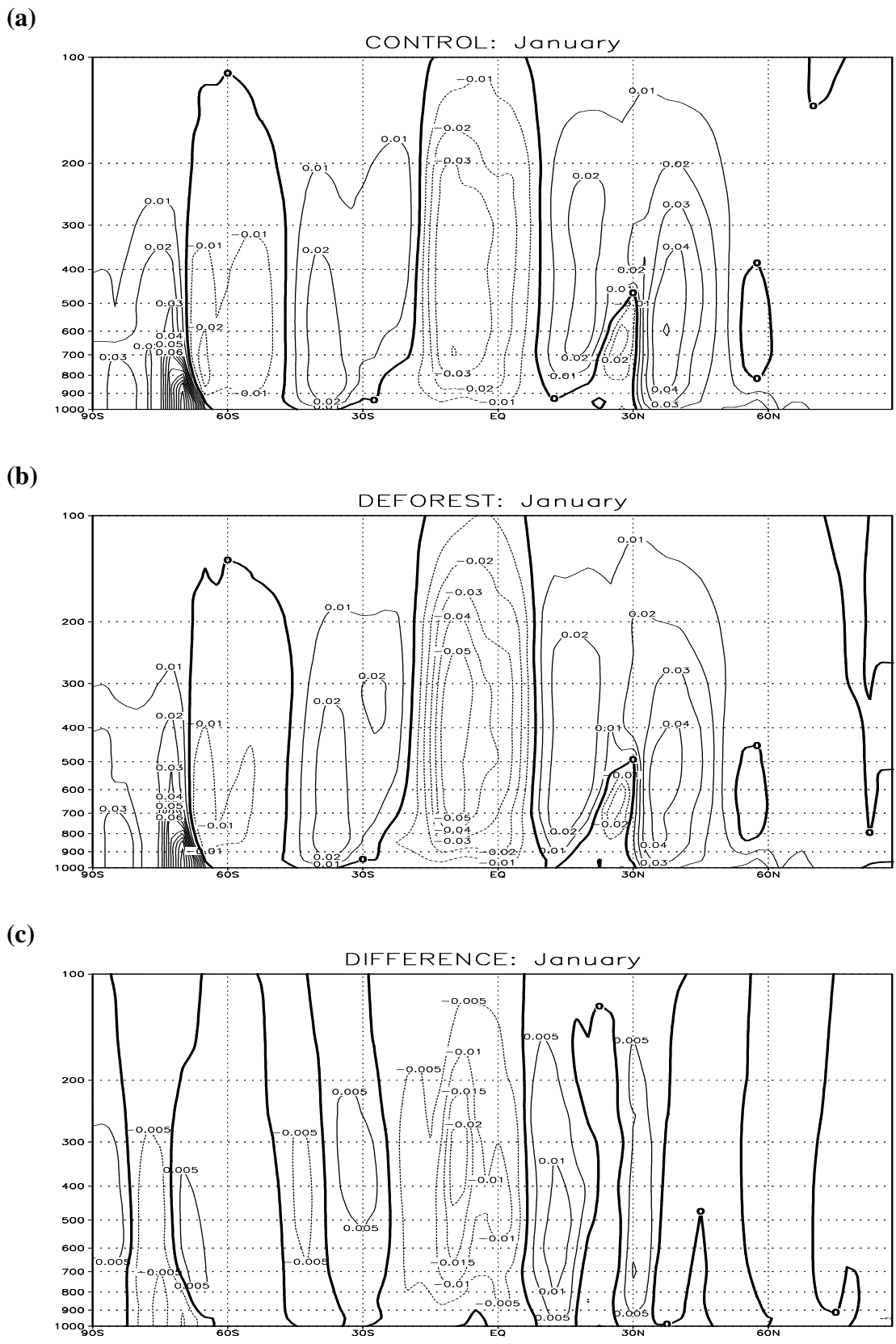
Figure 10.3: Change of Hadley circulation (zonal average of vertical velocity from 90°E to 150°E) (Pa/s) in January (composite from 10-case ensemble).
