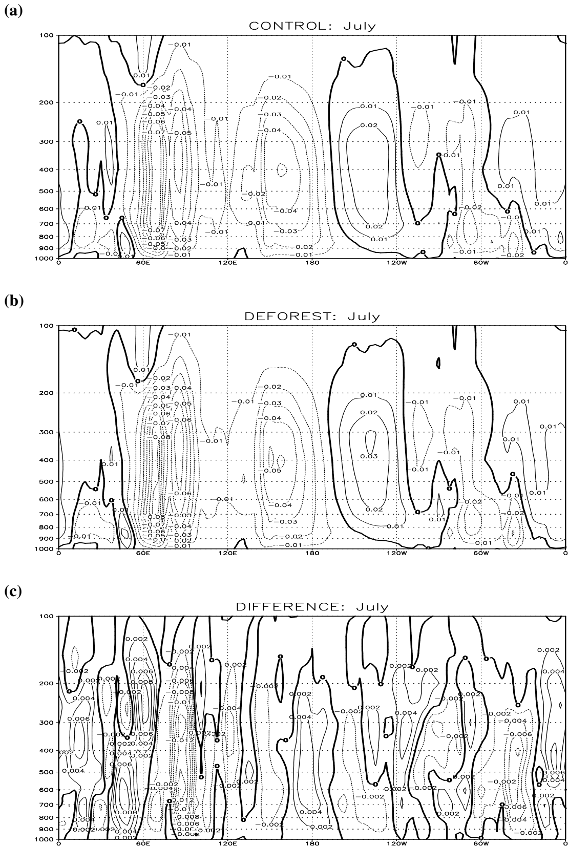
Figure 10.2: Change of Walker circulation (meridional average of vertical velocity from 15°S to 15°N) (Pa/s) in July (composite from 10-case ensemble).
