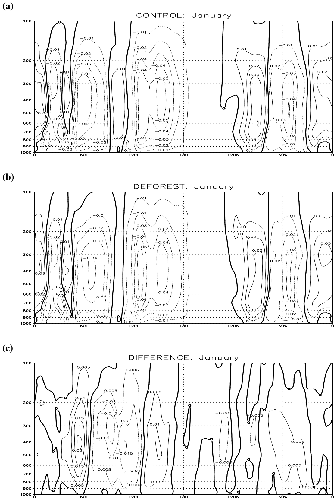
Figure 10.1: Change of Walker circulation (meridional average of vertical velocity from 15°S to 15°N) (Pa/s) in January (composite from 10-case ensemble).
