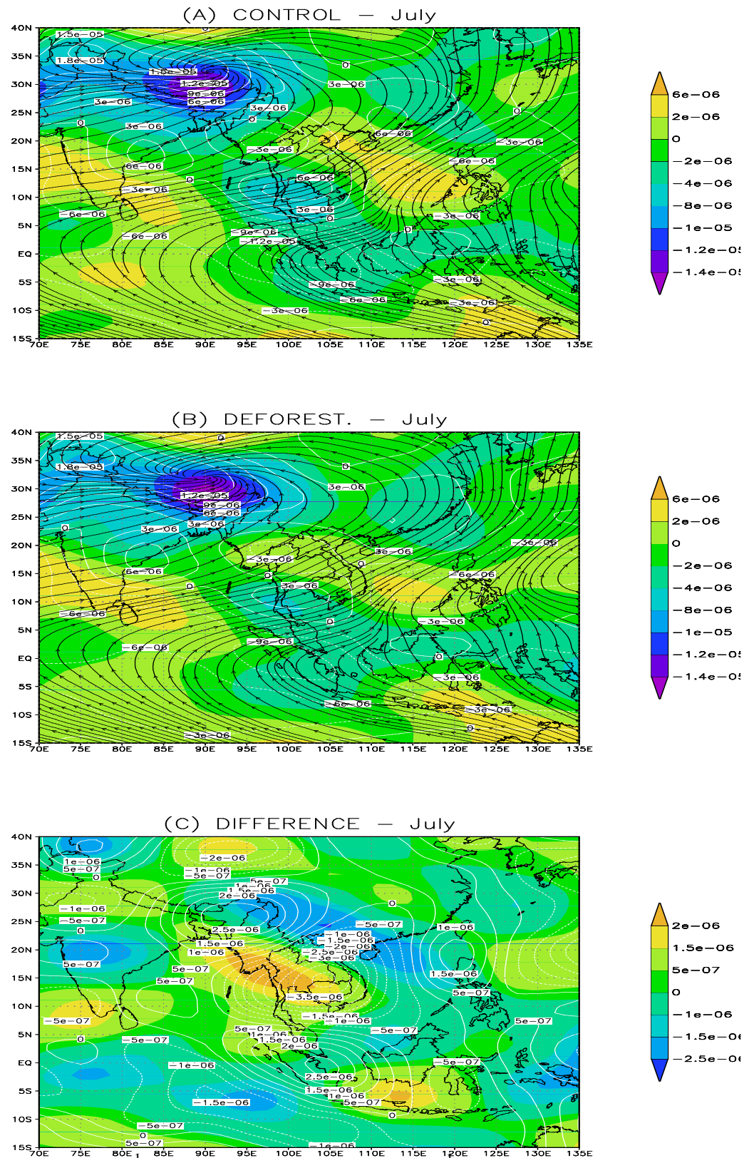
Figure 5.16: Divergence ( s^{-1} ) (colour shaded) and vorticity ( s^{-1} ) (white contour) near surface for July as given by the control (A) and deforestation (B) experiments. Changes (deforest.-control) are given in (C). (Associated streamlines are shown in the control and deforest. fields)
