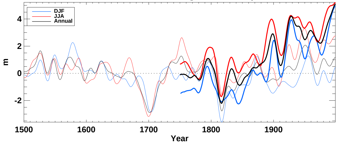
z850_ from hadcm3 averaged over Tropics land
