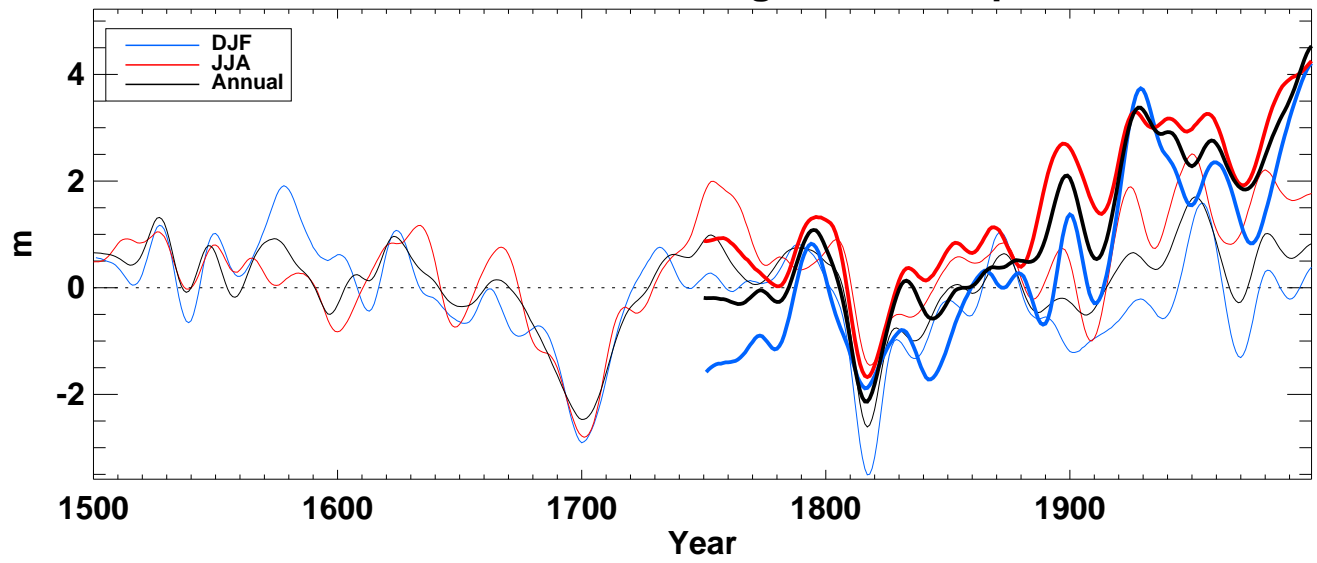
z850_ from hadcm3 averaged over Tropics full
