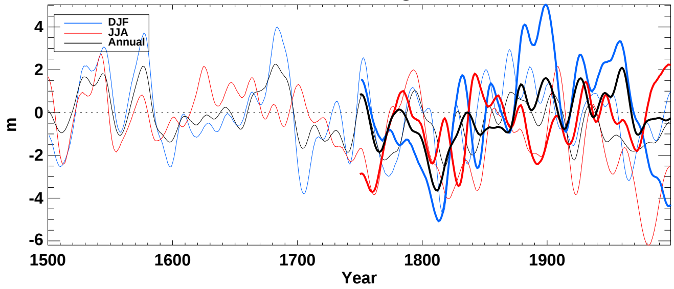
z850_ from hadcm3 averaged over SH land
