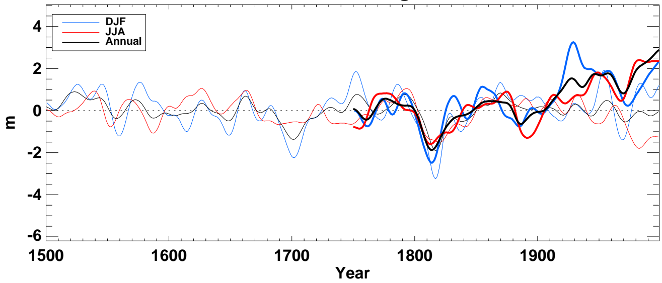
z850_ from hadcm3 averaged over SH full
