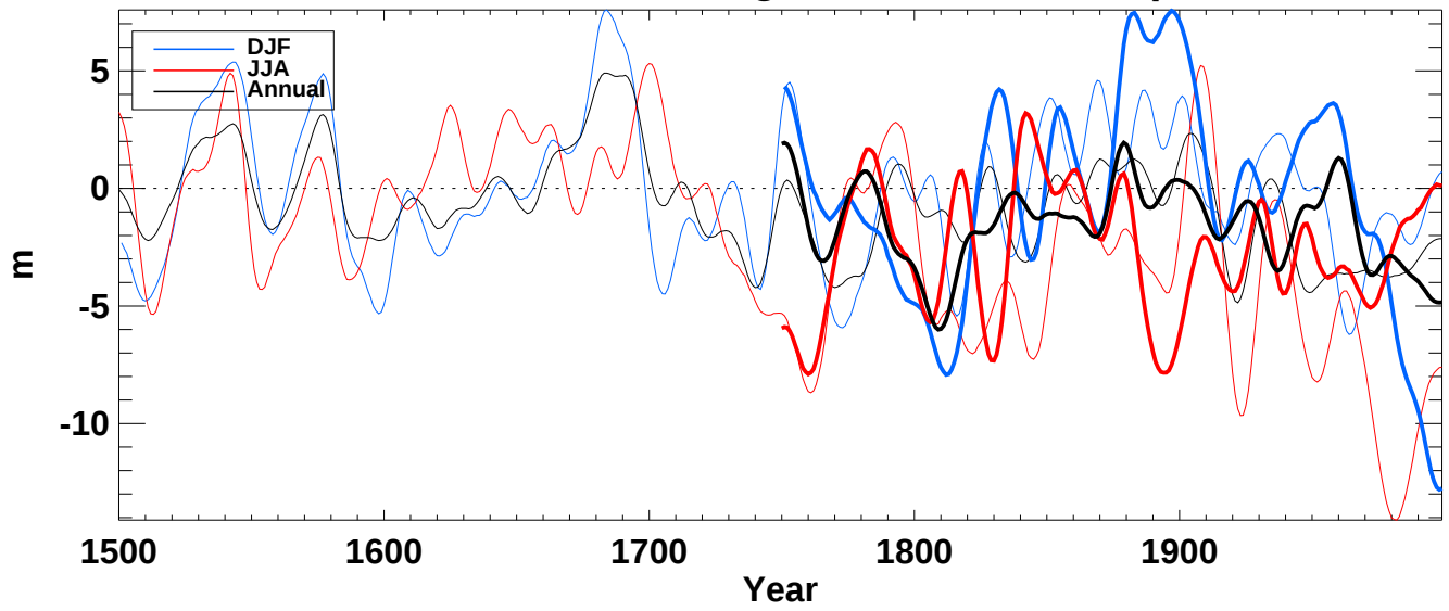
z850_ from hadcm3 averaged over S-extratropics land
