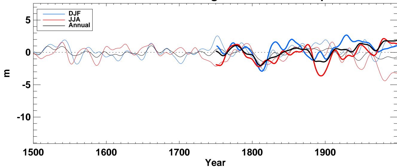
z850_ from hadcm3 averaged over S-extratropics full
