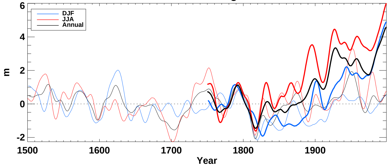
z850_ from hadcm3 averaged over NH land
