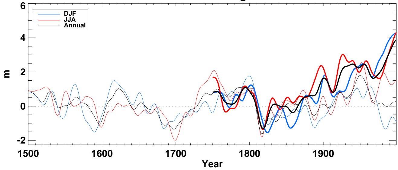
z850_ from hadcm3 averaged over NH full
