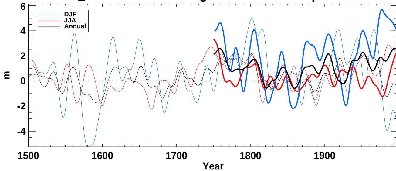
z850_ from hadcm3 averaged over N-extratropics ocean
