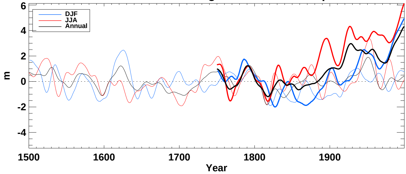
z850_ from hadcm3 averaged over N-extratropics land
