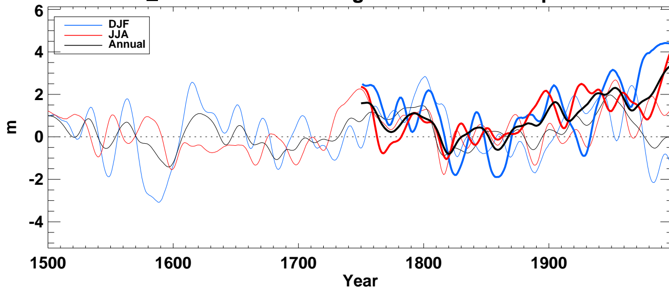
z850_ from hadcm3 averaged over N-extratropics full
