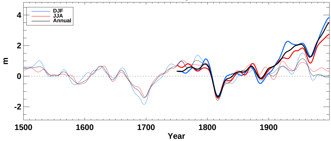
z850_ from hadcm3 averaged over Global ocean
