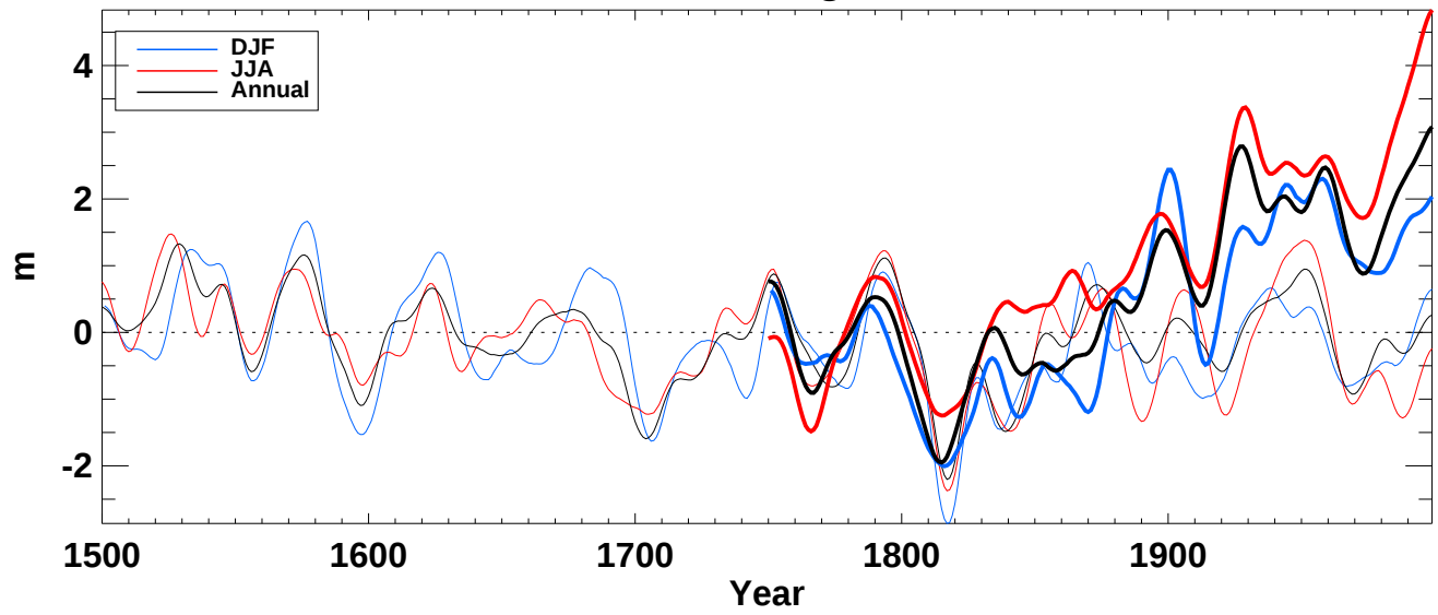
z850_ from hadcm3 averaged over Global land
